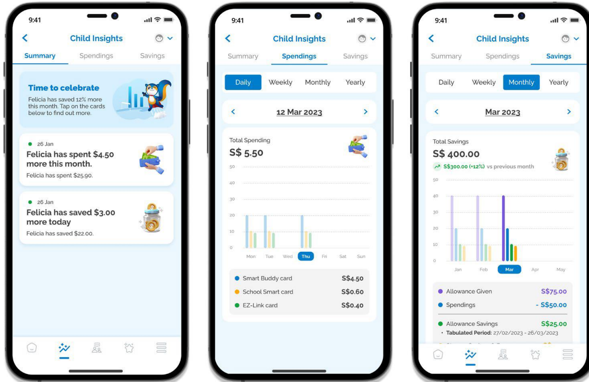
Figure 1: In-app Insights
